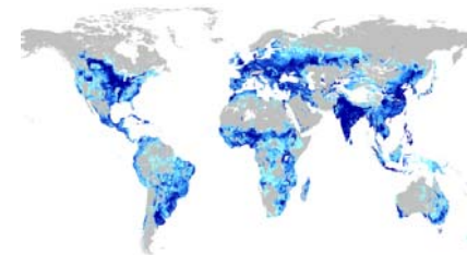
Spatially explicit
