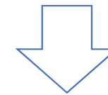
38 regions
